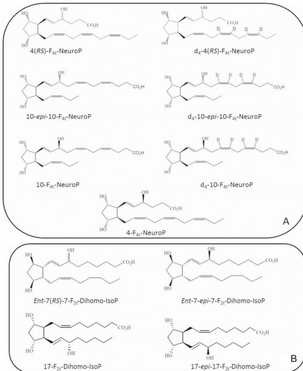
Figure 2 Chemical structures of F 4t -neuroprostanes, F 2t -dihomo-isoprostanes, and deuterated internal standards. A: F 4t -Neuroprostanes, B: F 2t -dihomo-isoprostanes.
