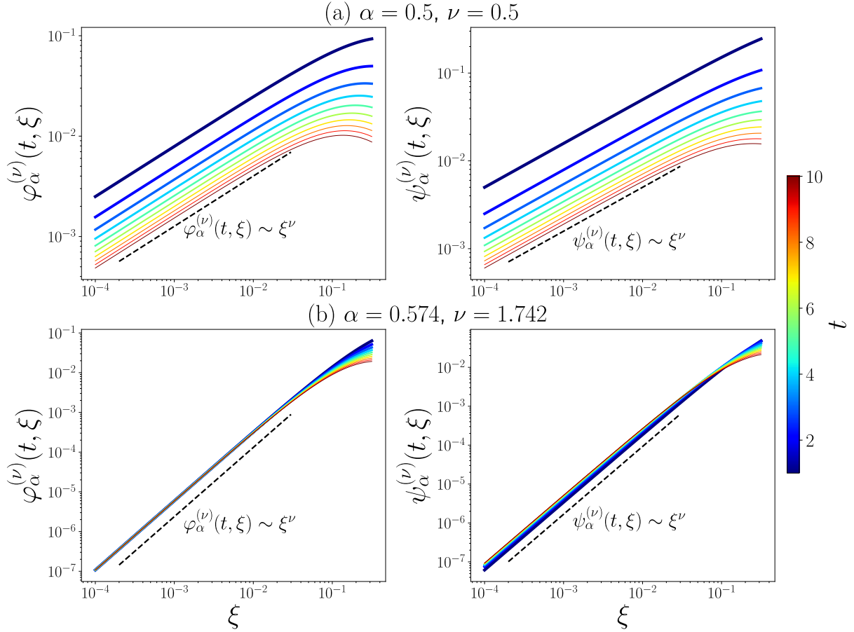
Figure 1: Discrete-time densities \varphi_\alpha^{(\nu)}(t, \xi) and \psi_\alpha^{(\nu)}(t, \xi) versus \xi for different values of t indicated in the colorbar t = 1, 2, \dots, 10 calculated using expression (14). For \xi \rightarrow 0 they approach a power-law \sim \xi^\nu indicated by dashed lines (See also in (14)).
