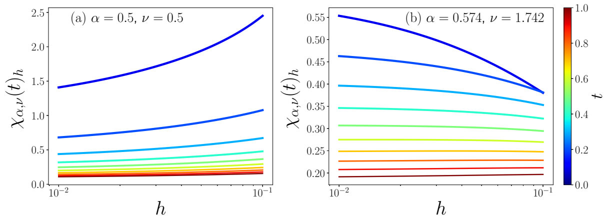
Figure 2: The plots show discrete-time waiting-time density \chi_{\alpha,\nu}(t)_h versus h for different times t . (a) \alpha = 0.5 and \nu = 0.5 , (b) \alpha = 0.574 and \nu = 1.742 . The colorbar represents the values of time t . The smaller h the more the GFPP Prabhakar waiting time density (2) is approached (See Eq. (20)).
