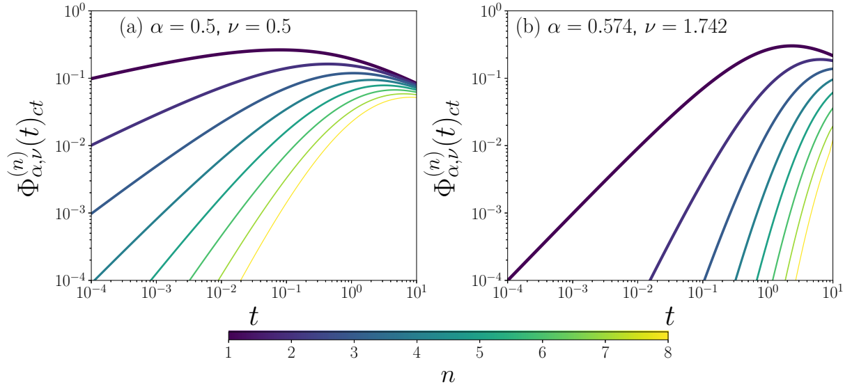
Figure 3: State probabilities \Phi_{\alpha,\nu}^{(n)}(t)_{ct} of the GFPP representing the continuous-time limit of the PDTP state probabilities versus t for different values of n . (a) \alpha = 0.5 and \nu = 0.5 , (b) \alpha = 0.574 and \nu = 1.742 . In the colorbar we represent the values n = 1, 2, \dots, 8 . The results were obtained numerically using \xi_0 = 1 with Eq. (52).
