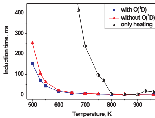
Figure 11. Dependencies of the induction time vs initial gas temperature. Methane stoichiometric mixture diluted by 76 % of argon, P=15 bar. Squares - reactions with O(^1D) are included, triangles - reactions with O(^1D) are not included, circles - all the deposited energy distributed to the heating with no active species production.
