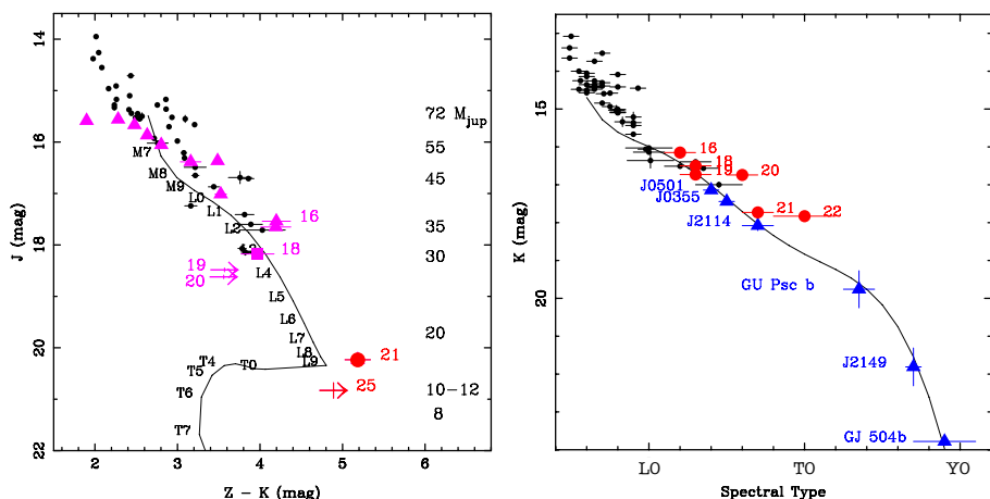
Fig. 2. UKIRT ZJK color–magnitude and spectral type–magnitude diagrams of confirmed Pleiades low-mass members (black and red dots). Calar 16, 18–22, and 25 are labeled. Previously known members of Bihain et al. (2010) are plotted as black dots. The magenta symbols stand for Zapatero Osorio et al. (2014a) candidates with Z photometry extracted from UKIDSS (triangles and arrows) and Sarro et al. (2014, square). Masses for an age of 120 Myr are labeled in the left panel. The field L and T dwarfs with an age close to that of the Pleiades (Delorme et al. 2012; Liu et al. 2013; Kuzuhara et al. 2013; Faherty et al. 2013; Naud et al. 2014; Zapatero Osorio et al. 2014b) are labeled and denoted by blue triangles. They are plotted as if they were located at 133.5 pc. Overlaid is the mean sequence of the field (solid line) produced by Dupuy & Liu (2012) taken to the Pleiades distance.
