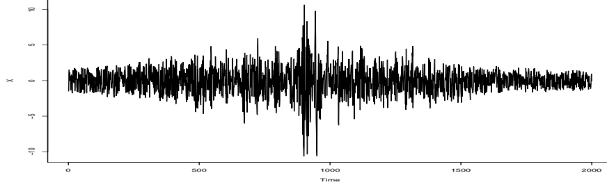
Figure 3: On trajectory of a tvARCH( \infty )-process for n = 2000
