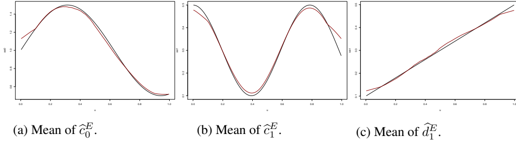
Fig 2: Paths of functions c_0, c_1, d_1 (in black), and the mean trajectories over 1000 replications of \hat{c}_0^E, \hat{c}_1^E and \hat{d}_1^E (in red) for n = 5000
