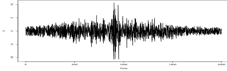
Fig 3: On trajectory of a tvARCH( \infty ) process for n = 2000
