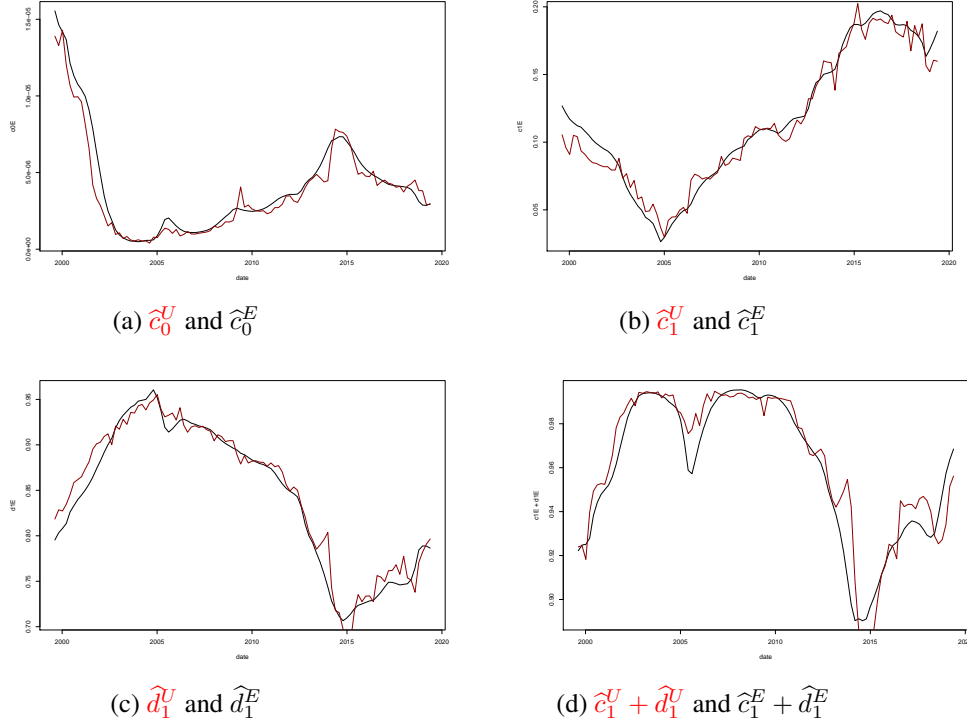
Fig 6: Estimators of c_0 , c_1 , d_1 and c_1 + d_1 for the log-returns of daily closing values of S&P500 index from July 1999 to July 2019
