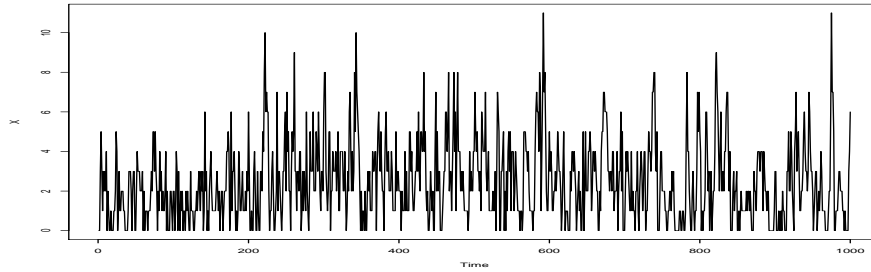
Fig 4: A trajectory of a tvINGARCH(1, 0) process for n = 1000
