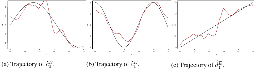
Fig 1: Paths of functions c_0, c_1, d_1 (in black), and a path of \hat{c}_0^E, \hat{c}_1^E and \hat{d}_1^E (in red) for n = 10000
