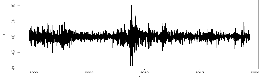
Fig 5: The log-returns of daily closing values of S&P500 index between July 1999 and July 2019
