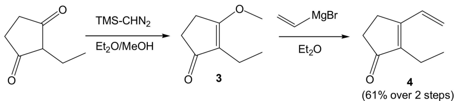
SCHEME 2 | Access to 2-ethyl-3-vinyl-cyclopentenone 4.
