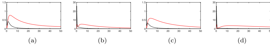
Fig. 2: Fast convergence of the velocity for different instances of \alpha, \beta, \lambda, e
