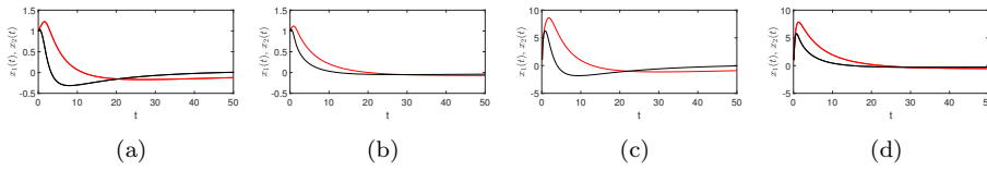
Fig. 1: Trajectories of (DIN-AVD) for different instances of the parameters \alpha, \beta, \lambda, e
