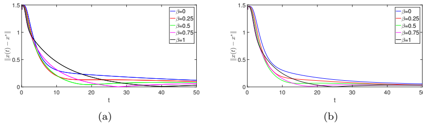
Fig. 3: Comparison of the iteration error \|x(t) - x^*\| for different instances of (DIN-AVD) without error
