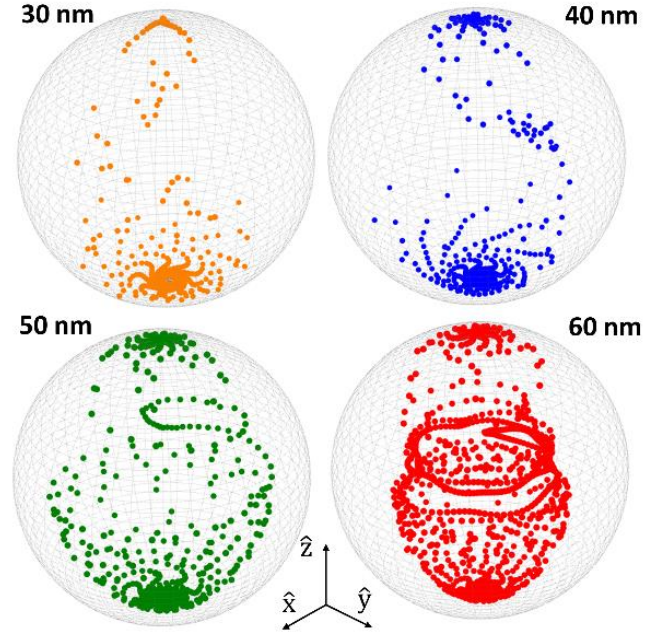
Fig. 4: Switching trajectories for layers of different thicknesses. The z-axis represents the \langle m_z \rangle and the basal plane (x and y axis) represents \langle m_{x,y} \rangle . The simulated data is contained in a macrospin sphere (radius 1). Results obtained for an applied bias of -1.25 V.
