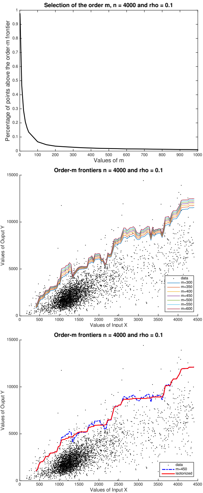
Figure 10: Final results for Case II: n = 4000 and \rho_{nts} = 0.10 .
