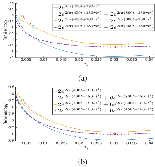
Fig. 2. (a): Computation of the Rényi entropy as a function of \sigma_s , with N = 512 , when f_1(t) = 2e^{2i\pi 400t + 180\pi t^2} and f_2(t) = 2e^{2i\pi 800t + 180\pi t^2} , the plain line is for f_1 only and the dashed line corresponds to f_1 + f_2 , then f_2 is replaced by 2e^{2i\pi 600t + 180\pi t^2} (plain line marked with stars) and then by 2e^{2i\pi 450t + 180\pi t^2} (plain line marked with circles), the squares correspond to the value of the Rényi entropy at \sigma_s = \frac{\sqrt{-\frac{\log(\epsilon)}{\pi}}}{\min(\phi'_1(t), \phi'_2(t) - \phi'_1(t))} ; (b): same as (a) except the amplitude of the second mode is 6.
