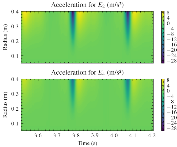
Figure 16: Acceleration of each structural node of the blade according to time (in \text{m/s}^2 ).
