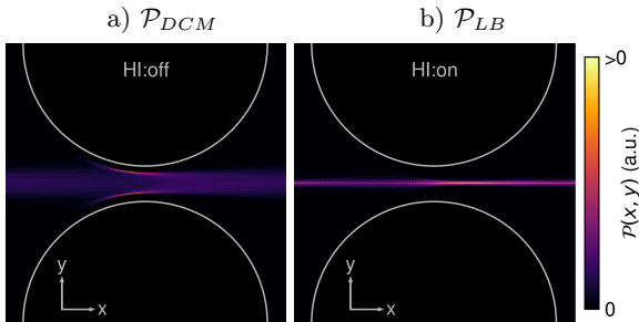
FIG. 10. Probability distribution \mathcal{P}(x, y) of the position of a single swimmer in a unit cell for \Gamma = 1 , \tau_{\text{ph}} \approx 8a/V_0 and \theta_\ell = 0 . a) Without hydrodynamic interactions (DCM simulations), the interaction between swimmers and pillars is collision based, leading to a high probability to find particles at the contact positions near the pillars. b) For simulations with HI (LB simulations), we find pronounced focusing between the pillars. This indicates that hydrodynamics help the swimmers to avoid collisions with the obstacles.
