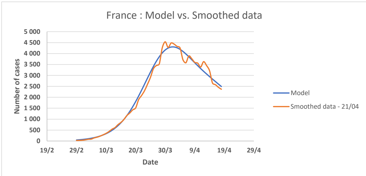
Figure 11: Comparison between the smoothed data of the number of detected cases of COVID-19 in
