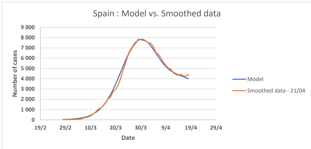
Figure 13: Comparison between the smoothed data of the number of detected cases of COVID-19 in Spain and our model
