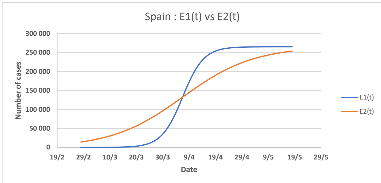
Figure 8: Graph of functions E_1(t) and E_2(t) for Spain, E_1 describing the epidemic without a lockdown (in blue), E_2 with a lockdown from the start (in red).
