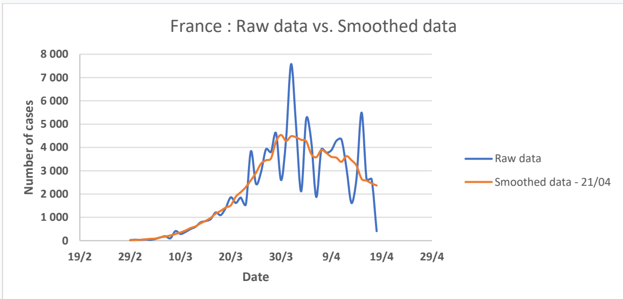
Figure 2: Raw data and smoothed data over 7 days of the number of detected cases of COVID-19 in France in 2020 according to [21]
