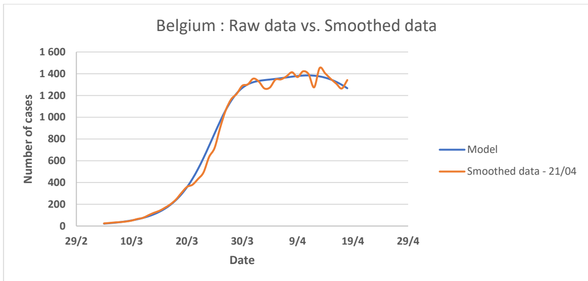
Figure 10: Comparison between the smoothed data of the number of detected cases of COVID-19 in Belgium and our model
