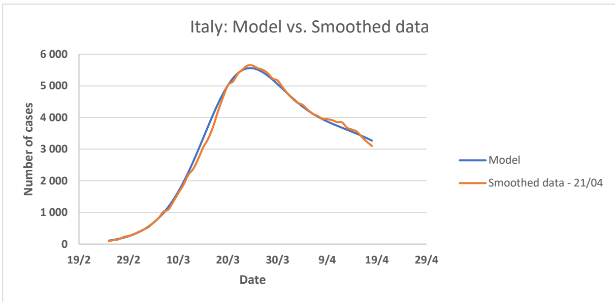
Figure 12: Comparison between the smoothed data of the number of detected cases of COVID-19 in
