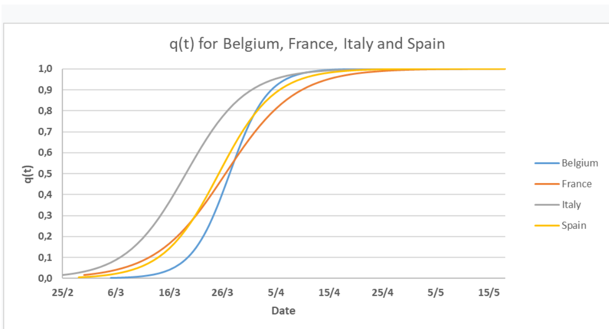
Figure 9: Comparison of the functions q(t) for Belgium, France, Italy, and Spain. The parameters were optimized by machine learning
