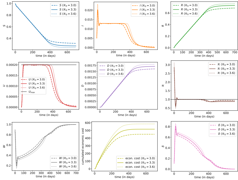
Figure 7: Evolution of states with optimal controls (\delta, 0, 0) – without any testing – for three different values of \mathfrak{R}_0 . The plain line is the benchmark scenario discussed in Section 3.2; the dashed line corresponds to a smaller value of \mathfrak{R}_0 ( -0.3 ) while the dotted line corresponds to a larger value of \mathfrak{R}_0 ( +0.3 ).
