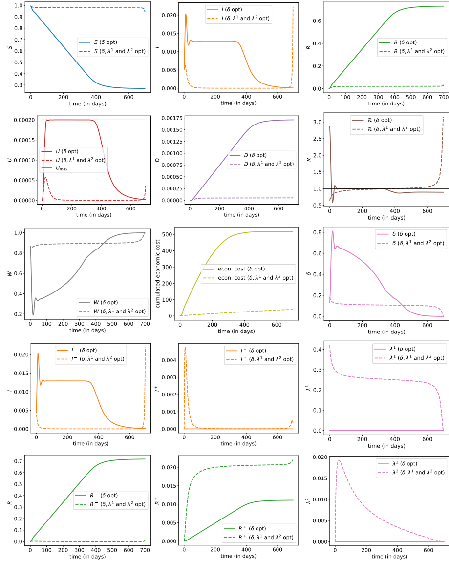
Figure 17: Evolution of states with optimal controls (\delta, \lambda^1, \lambda^2) , where the plain line corresponds to the benchmark scenario (\delta, 0, 0) discussed in Section 3.2 (plain line); and evolution with joint optimal controls (\delta, \lambda^1, \lambda^2) (dashed line).
