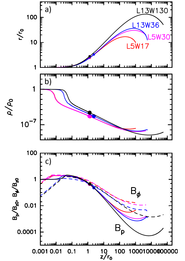
Fig. A.2. Variation of a : radius, b : density \rho , and c : poloidal and toroidal magnetic field (in solid and dashed curves respectively) along a magnetic wind surface as a function of z/r_0 , for the four computed MHD DW solutions. The Alfvén point for each solution is plotted as a filled dot. Quantities are normalized by the mid-plane value of radius, density, and vertical magnetic field B_{z,0} at r_0 . The latter are related to the dimensional parameters of the system through \rho_0 \simeq \dot{M}_{\text{acc}}(r_0)/(4\pi r_0^2 V_{K,0} \epsilon^2 m_s) and B_{z,0}^2 \simeq \mu \dot{M}_{\text{acc}}(r_0) V_{K,0}/(r_0^2 m_s) , where m_s \simeq 1-2 is the Mach number of the accretion flow (Combet & Ferreira 2008).
