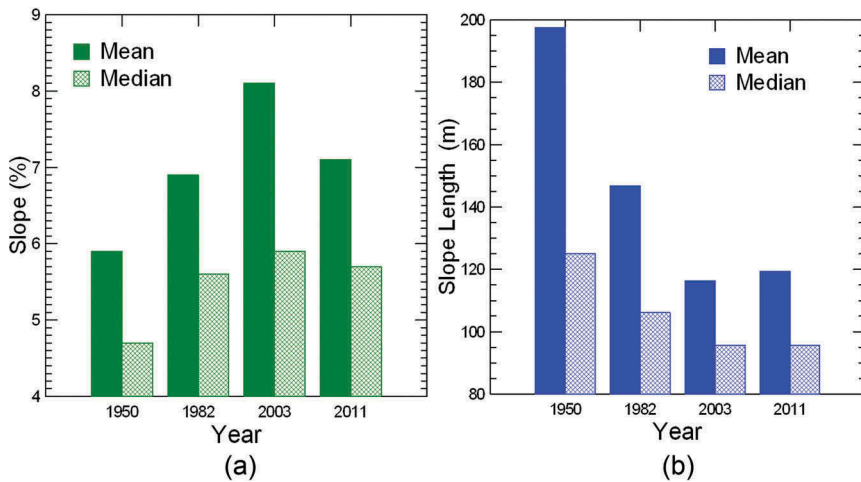
Figure 5. (a)Changes in mean and median slope inclination over time. b Changes in mean and median slope length over time.
