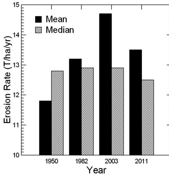
Figure 6. Changes in mean and median soil erosion rates over time.
