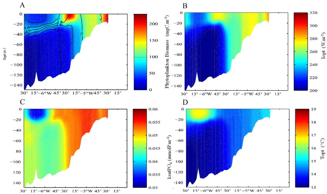
Fig. 6. Vertical distribution of (A) total modeled phytoplankton biomass ( mgC \cdot m^{-3} ) along the 48^{\circ}N transect (Fig. 4, B) with the surface isotherms ( ^{\circ}C ). Vertical structure of September monthly average of functional traits weighted by phytoplankton biomass: (B) light optimum ( W \cdot m^{-2} ), (C) phosphorus half saturation constant ( mmolP \cdot m^{-3} ) and (D) temperature optimum ( ^{\circ}C ).
