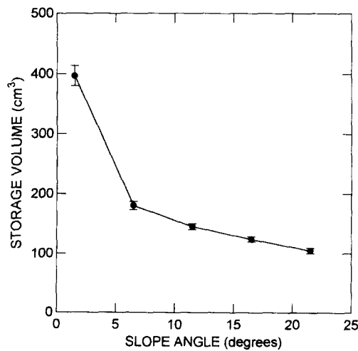
Fig. 4. Decreasing surface storage volume with increasing slope angle (error bars are \pm 1 standard error).
