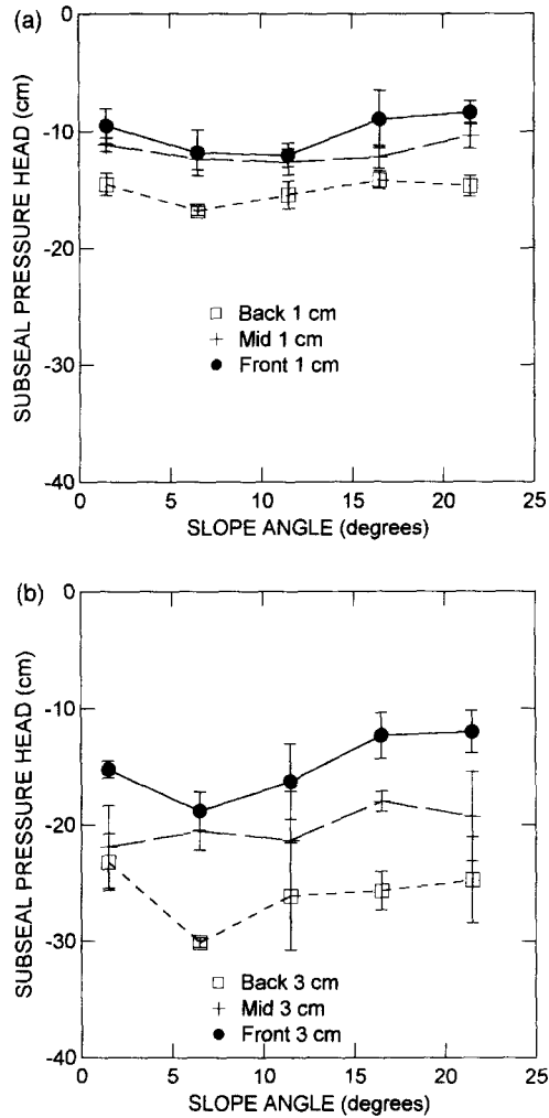
Fig. 2. (a) Mean subseal pressure heads at 1 cm depth for all slope angles (error bars are \pm 1 standard error). (b) Mean subseal pressure heads at 3 cm depth for all slope angles (error bars are \pm 1 standard error).
