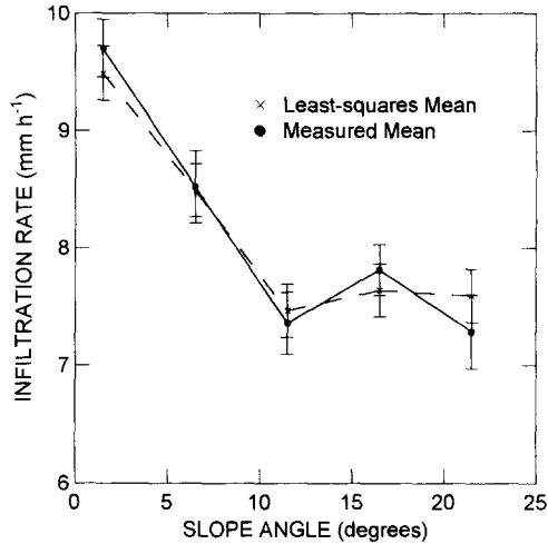
Fig. 1. Decreasing mean measured and least-squares mean final infiltration rates with increasing slope angle (error bars are \pm 1 standard error).
