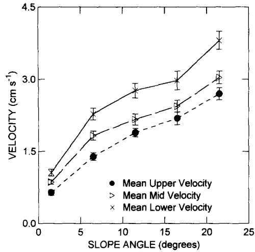
Fig. 3. Overland flow velocity increases with both slope angle and position within the soil tray (error bars are \pm 1 standard error).
