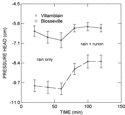
Fig. 6. Increase in pressure head with the addition of runoff (error bars are \pm 1 standard error).
