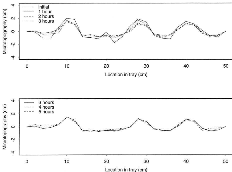
Fig. 2. Changes in microtopography for Blossville showing the progressive flattening of the surface with time (a) during first 3 h rainfall simulation, (b) during final 2 h rainfall simulation.
