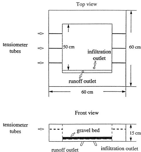
Fig. 1. Experimental soil tray showing surrounding buffer area, tensiometer locations, and infiltration and runoff outlets.
