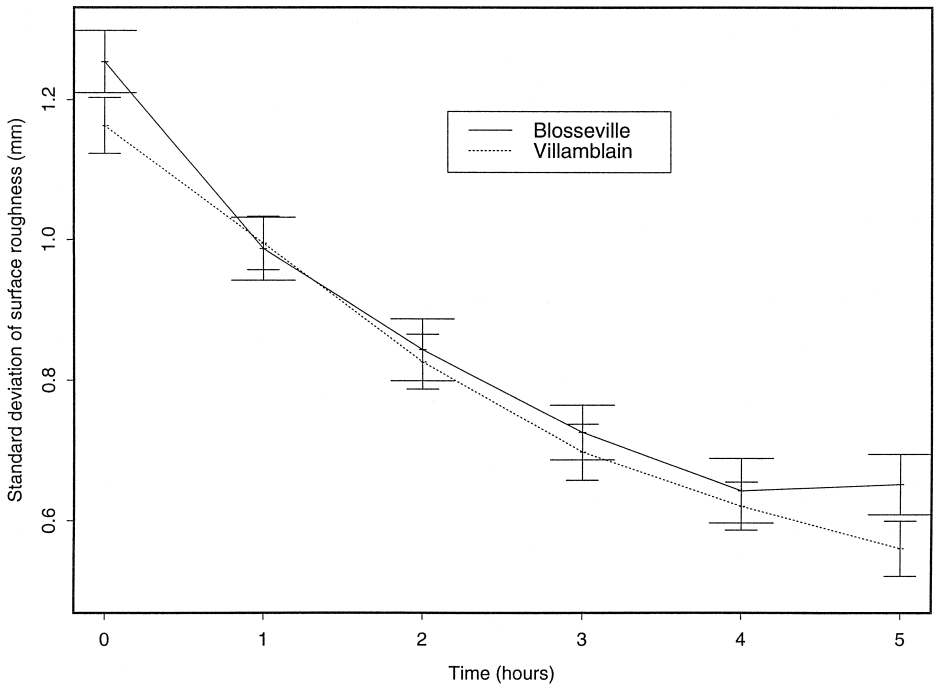
Fig. 4. Changes in standard deviation of surface roughness during 5 h of rainfall simulation (error bars are \pm 1 standard error).
