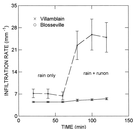
Fig. 7. Increase in infiltration rate with the addition of runoff (error bars are \pm 1 standard error).
