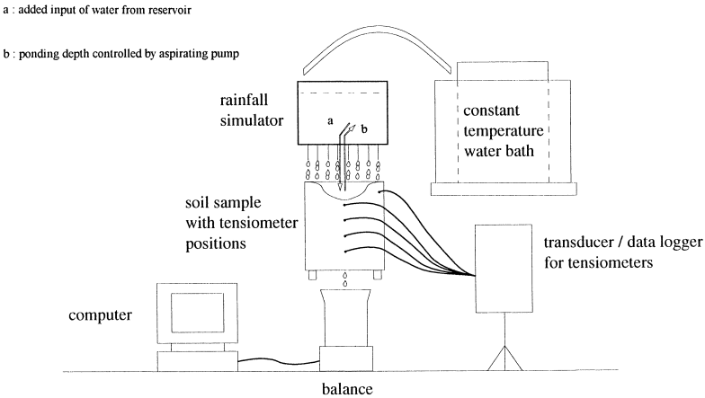
Fig. 2. Experimental setup: water at constant temperature was supplied to the rainfall simulator and directly into the depression under deep ponding. Ponding depth was controlled by an aspirator pump, and the water flux was measured continuously.
