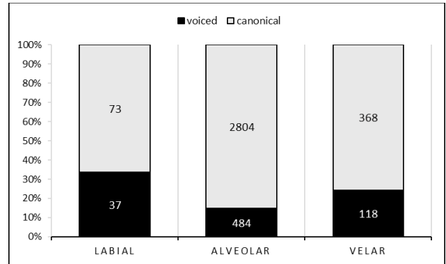
Figure 7: Percentage (and counts) of voiced codas preceding voiced consonants as a function of place of articulation
