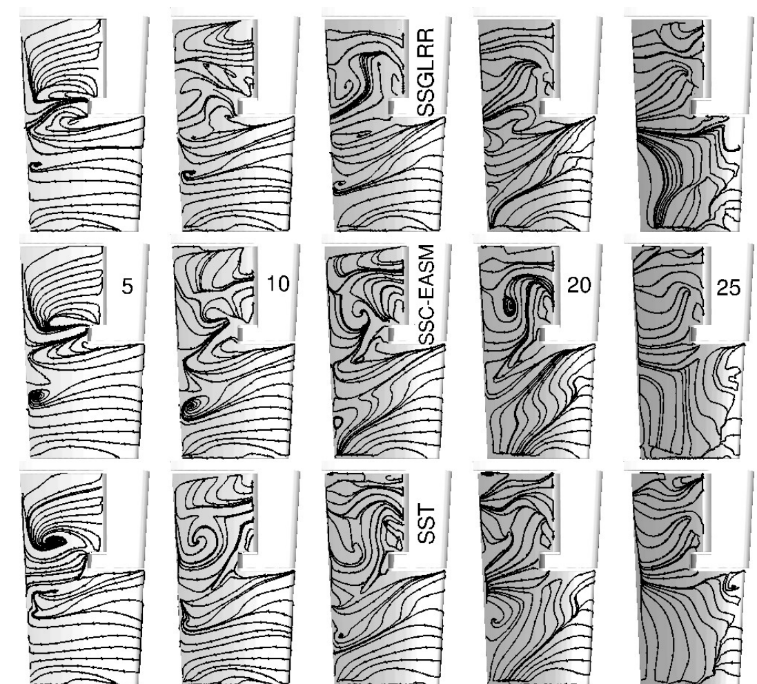
Figure 1. Wall limiting streamlines
