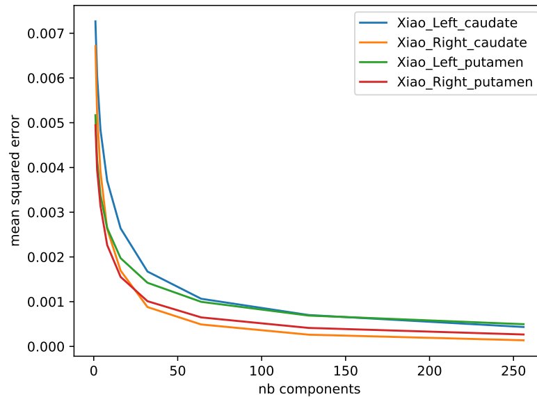
Figure 3: Reconstruction mean squared error of PCA compression on test set for left caudate nucleus (blue), right caudate nucleus (orange), left putamen (green) and right putamen (red), with various number of components kept.
