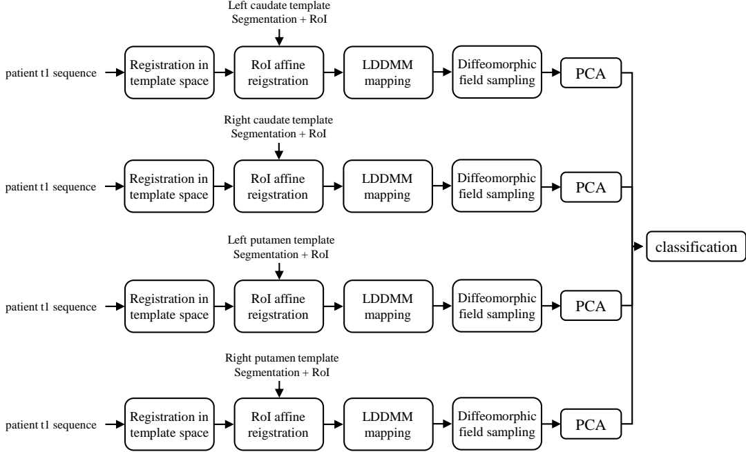
Figure 1: Pipeline proposed and tested in this study.
