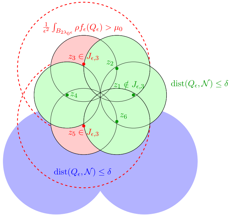
Figure 2: Second covering argument: Find balls, where \frac{1}{\epsilon^2} \int \rho f_\epsilon(Q_\epsilon) is large
