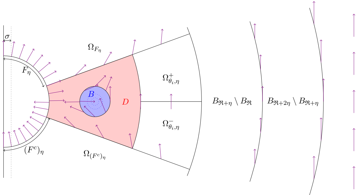
Figure 4: Partition of \Omega' into regions for the construction of Q_\epsilon (arrows show \mathbf{n}^\epsilon )
