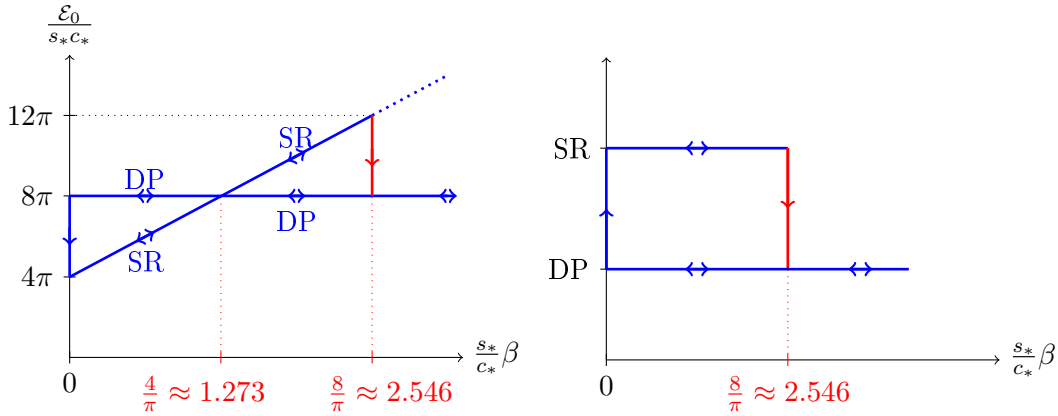
Figure 6: Left: Plot of the energy of the dipole and Saturn ring as a function of \frac{s_*}{c_*}\beta . Right: Hysteresis induced by changing \frac{s_*}{c_*}\beta
