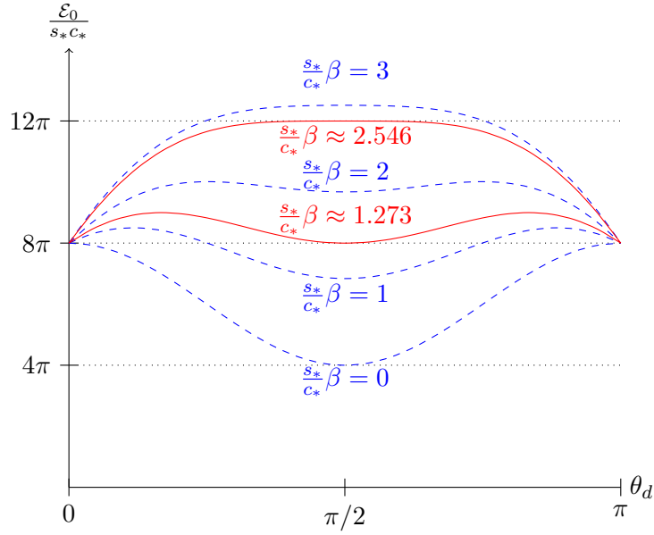
Figure 5: Plot of the energy \mathcal{E}_0 for different values of \beta s_* as a function of the angle \theta_d
