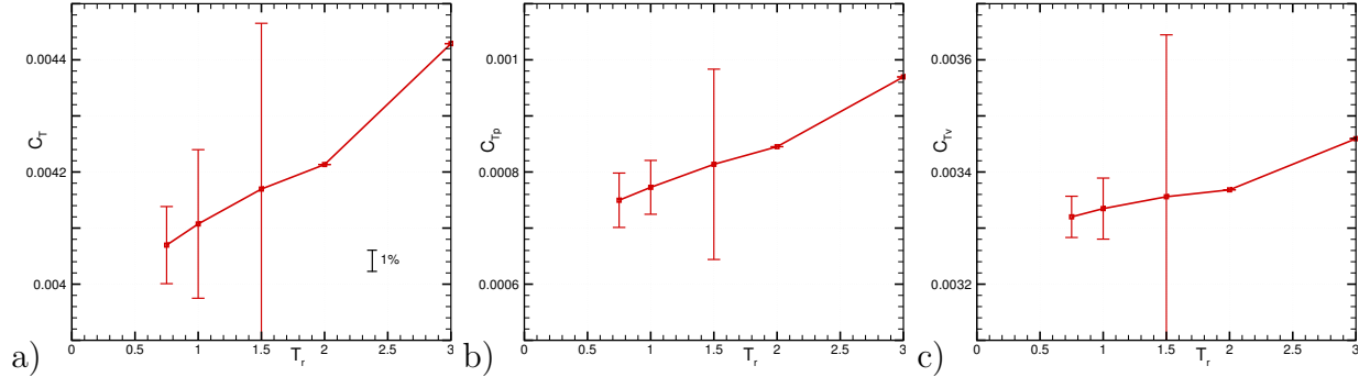
Figure 7: Grid convergence for the KVLCC2: resistance coefficient C_T (a), pressure and viscous resistance coefficients C_{Tp} (b) and C_{Tv} (c), with uncertainty computed using all the coarser grids available. The scale of the axes is the same for the three graphs.
