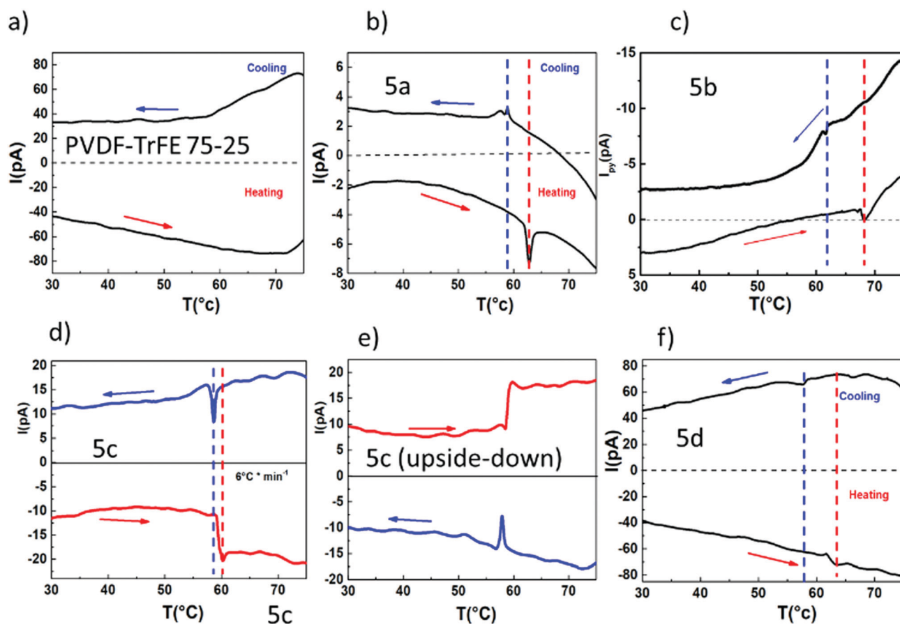
Fig. 7 (a) Pyroelectric discharge cycles for the pure 75/25% P(VDF-TrFE) polymer. (b–f) Pyroelectric discharge cycles for composites 5a–5d. The arrows indicate heating and cooling. Dotted lines show the SCO related discharge peaks for cooling (left) and heating (right).
