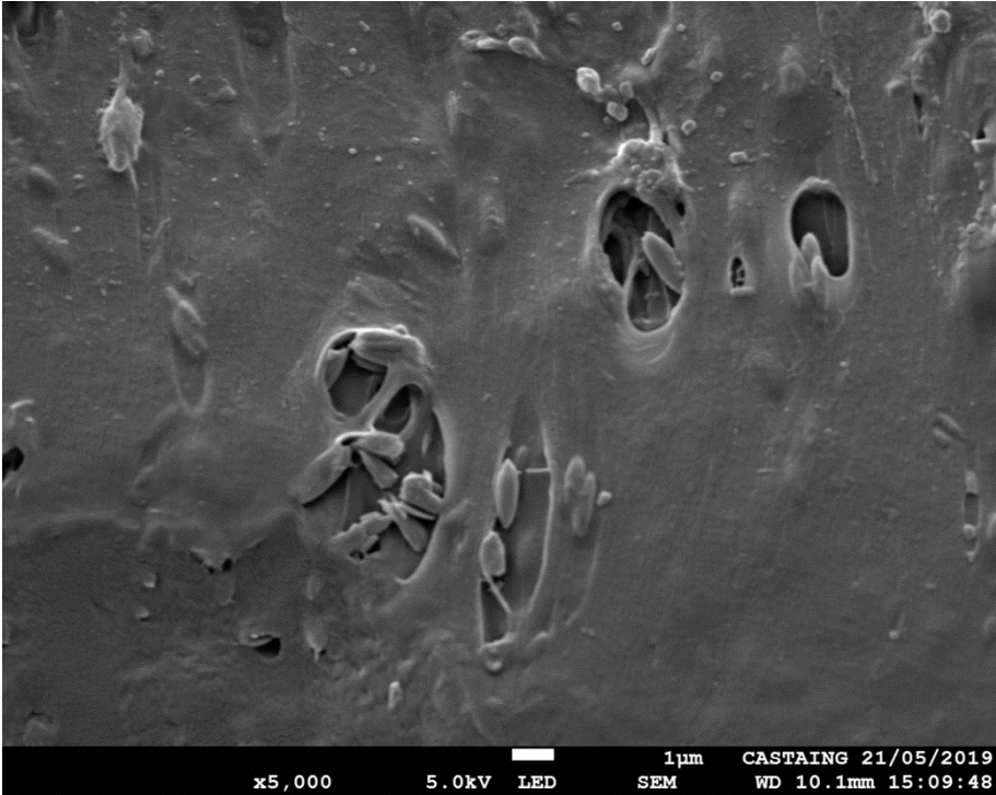
Figure S1: SEM images of the composite 1a cross-section.
