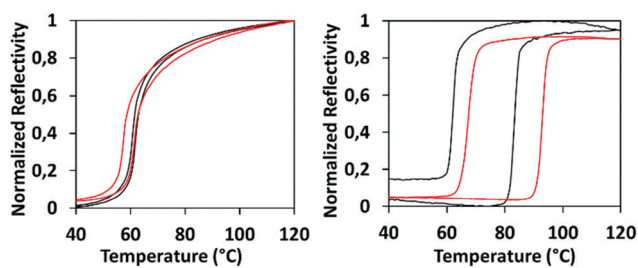
Fig. 6 Variable temperature optical reflectivity measurements for the bulk compounds 1 and 5 (in black) and the corresponding composite samples 1a and 5a (in red).
