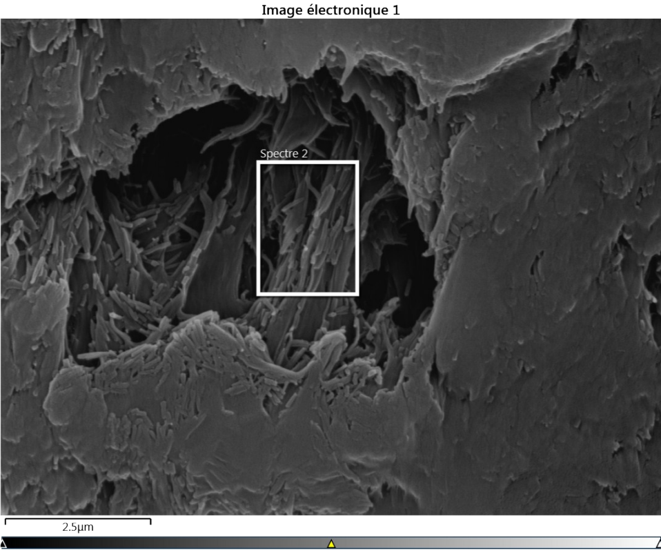
Figure S4: SEM coupled EDX analysis of two randomly selected areas for composite 4a .
