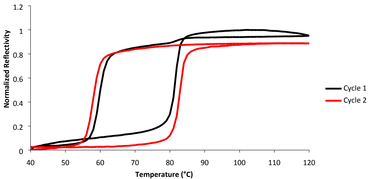
Reflectivity Measurement of Composite 3a
