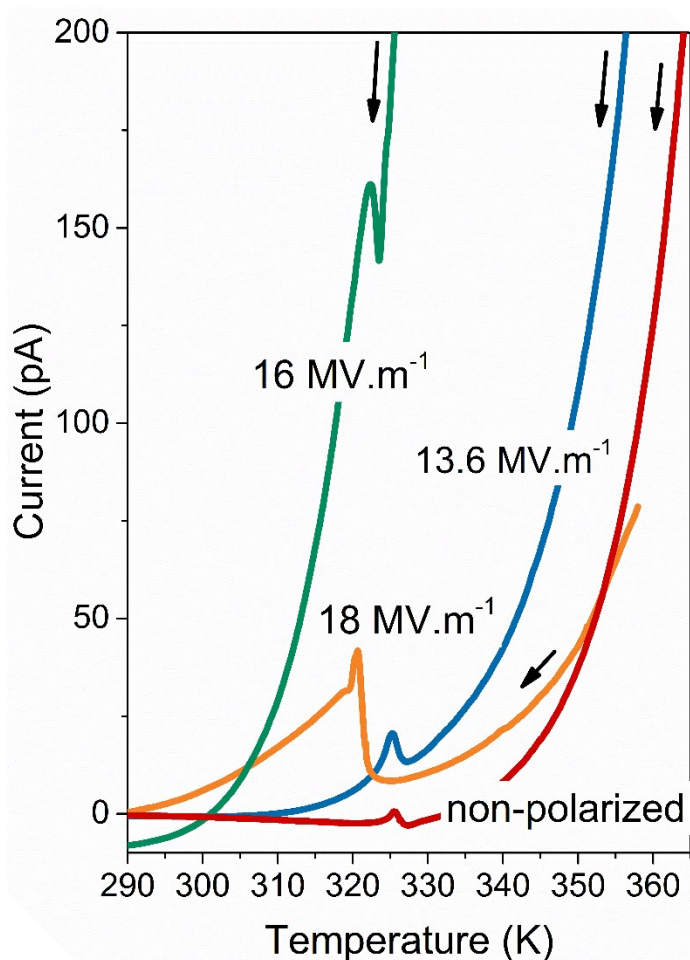
Figure S12: Pyroelectric discharge cycle for composite 2a with different polarization intensities:
