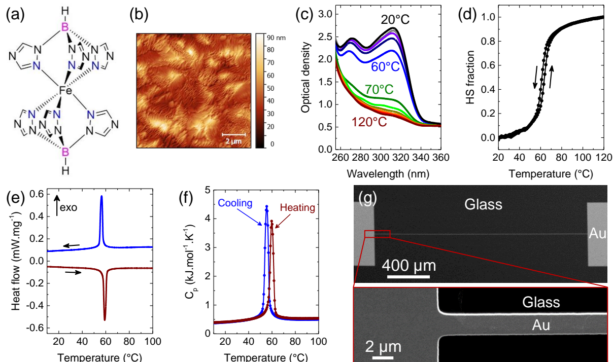
Figure 1. (a) Molecular structure of the complex 1 . (b) Atomic force microscopy (AFM) topography image of a 900-nm-thick film of 1 . (c) Optical absorbance spectra of the film acquired at different selected temperatures in the heating mode between 20 °C (LS state) and 120 °C (HS state). (d) Temperature dependence of the fraction of HS molecules extracted from the variation of the optical density. (e) Differential scanning calorimetry (DSC) analysis of the bulk powder of 1 acquired at a scan rate of 2 °C.min -1 . (f) Thermal evolution of the molar heat capacity ( C_p ) of 1 , showing the excess C_p associated with the spin-transition phenomenon. (g) Scanning electron microscopy (SEM) image of a 2-mm-long, 2- \mu\text{m} -wide gold wire used as a micro-heater on a glass substrate.
