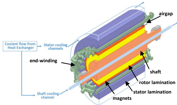
Figure 9: High specific power electric motor section
