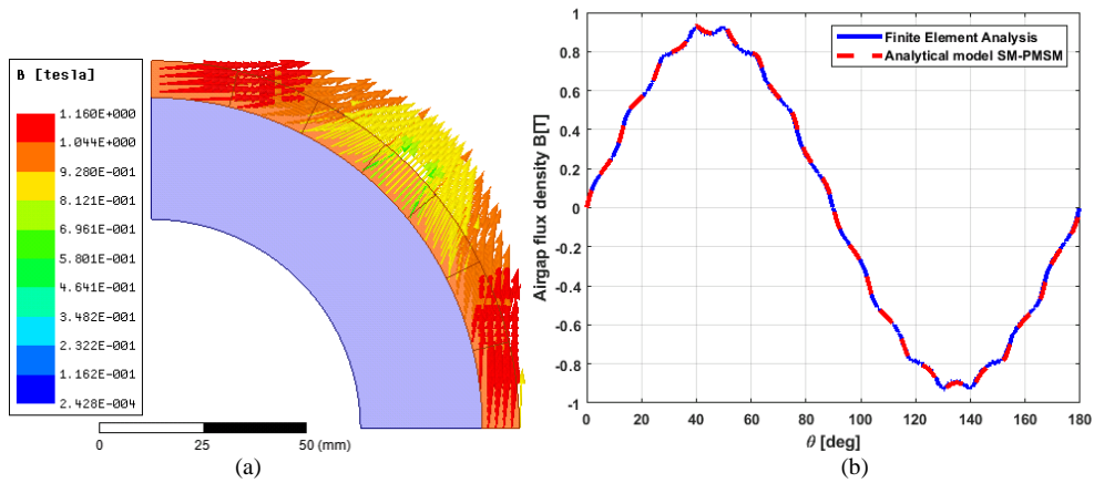
Figure 7: (a) Halbach segmented permanent magnet, (b) Airgap flux density
