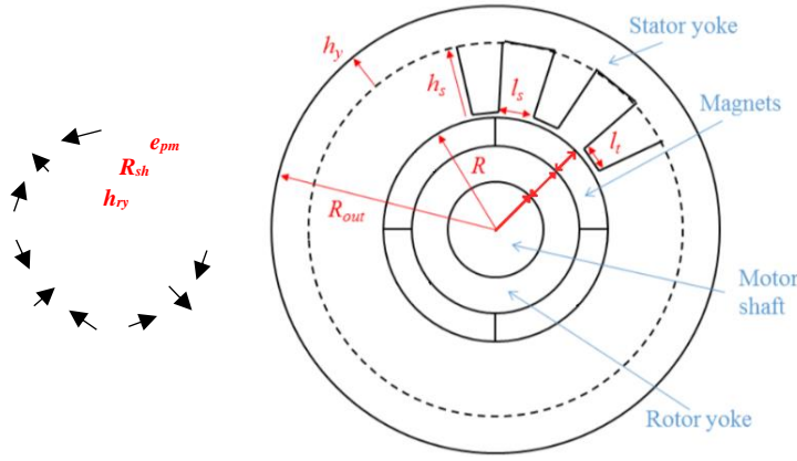
Figure 2: Sizes given by SM-PMSM Tool
