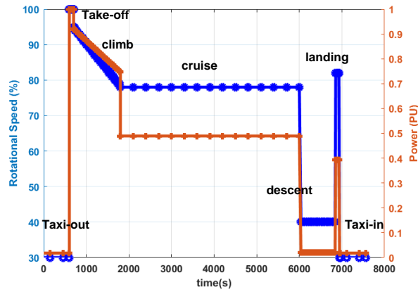
Figure 4. Mechanical power and rotational speed of propeller vs time
