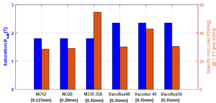
Figure 5: Comparison between electrical steels
