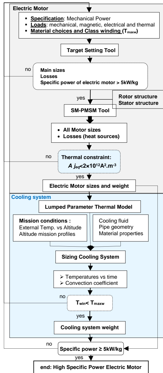
Figure 3: Interaction between Electro-thermal models for sizing high specific electric motor with its cooling system
