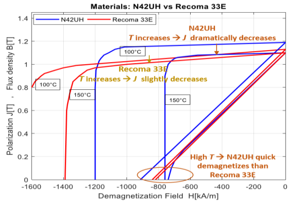
Figure 6: Comparison between NdFeB (N42UH) and SmCo (Recoma 33E)
