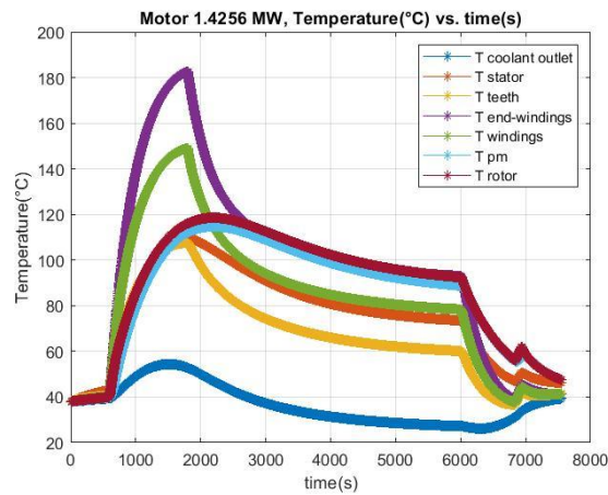
Figure 13: Temperature evolution during flight mission in the designed high specific power electric motor.
