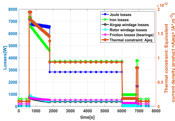
Figure 10: Losses profiles vs time
