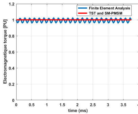
Figure 11: Electromagnetic torque validation
