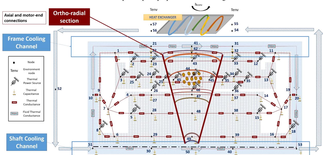
Figure 12: Axial and ortho-radial sections of half SM-PMSM electric motor including its cooling system with LPTM nodes locations, and axial and motor-end connections.
