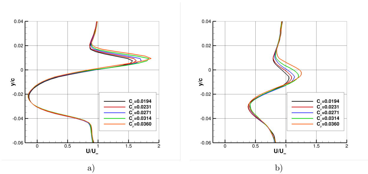
Figure 12. Y profiles for the discrete squared jet control configuration at z/c = 0 and: a) x/c = 1.01 b) x/c = 1.05
