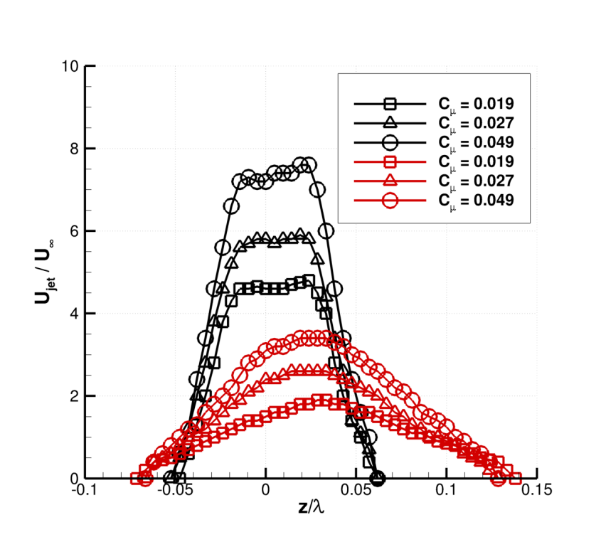
Figure 3. Mean jet control profiles at x/c=0.965 and y/c=0 (black lines) and at x/c=1.01 and y/c=0.0075 (red lines)
