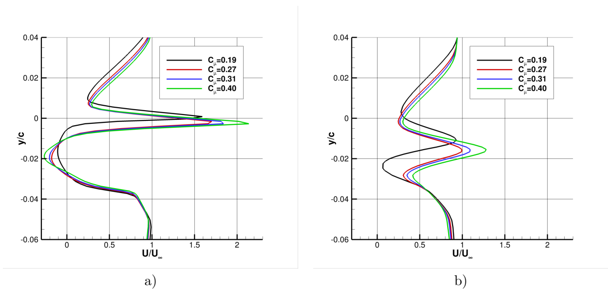
Figure 13. Y profiles for the slotted jet control configuration at: a) x/c = 1.01 b) x/c = 1.05
