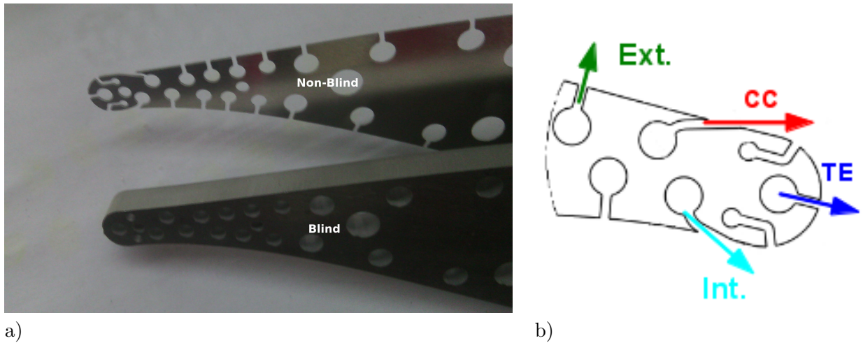
Figure 2. a) Samples of a blind and a non-blind NACA65 4 -421-CC profile, b) Examples of jet control possibilities from this design: blowing for Circulation Control (CC: red arrow), Trailing Edge blowing (TE: blue arrow), Intrados blowing (Int: cyan arrow), Extrados blowing (Ext.: green arrow)
