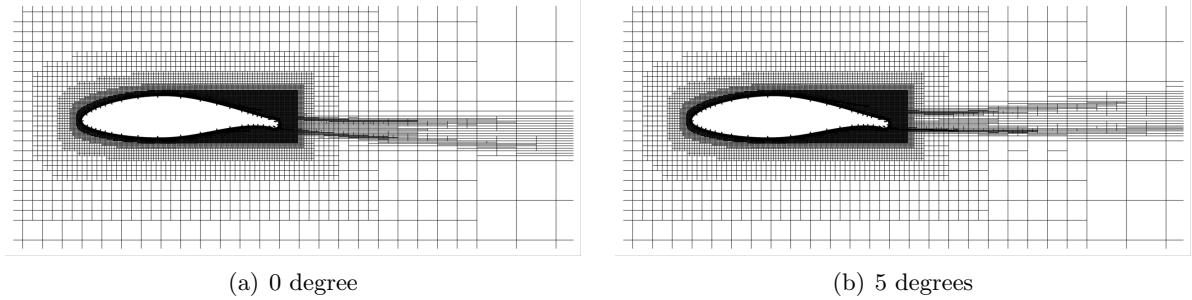
Figure 5. Refined meshes
