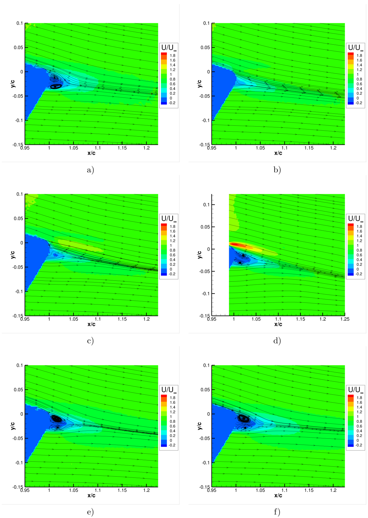
Figure 14. 2D-2 components PIV planes in the transverse direction of the discrete squared jet configuration, for C_{mu} = 0.027 : a) z/\lambda = 0.43 b) z/\lambda = 0.33 c) z/\lambda = 0.14 d) z/\lambda = 0 e) z/\lambda = -0.19 f) z/\lambda = -0.33 .
