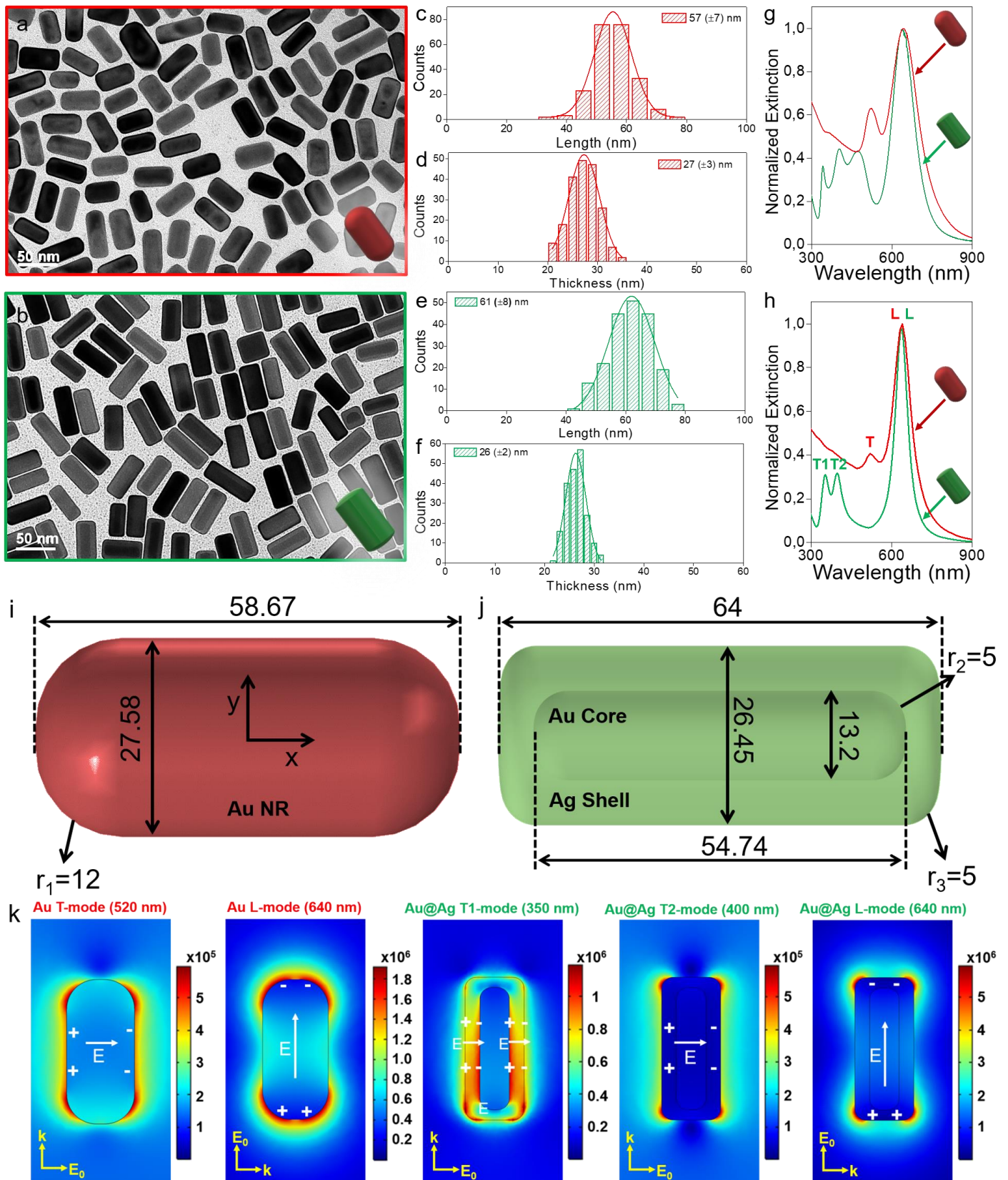
Figure 1. (a, b) TEM images, (c-f) size histograms, (g) experimental, and (h) theoretical extinction spectra of the Au NRs (red) and the Au@Ag NRs (green). Morphological features for the simulation of (i) Au NRs, and (j) Au@Ag NRs (being r_1 , r_2 and r_3 the radii of curvature for rounding edges). (k) Near-field enhancement maps of the plasmonic modes of the Au and Au@Ag NRs.
