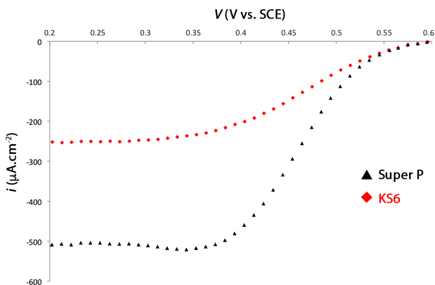
Figure 6. Polarization curve of an ABTS/laccase modified electrode in phosphate buffer solution (pH 5, 0.1 M) under O 2 . Comparison between carbon powders KS6 and Super P ® .
