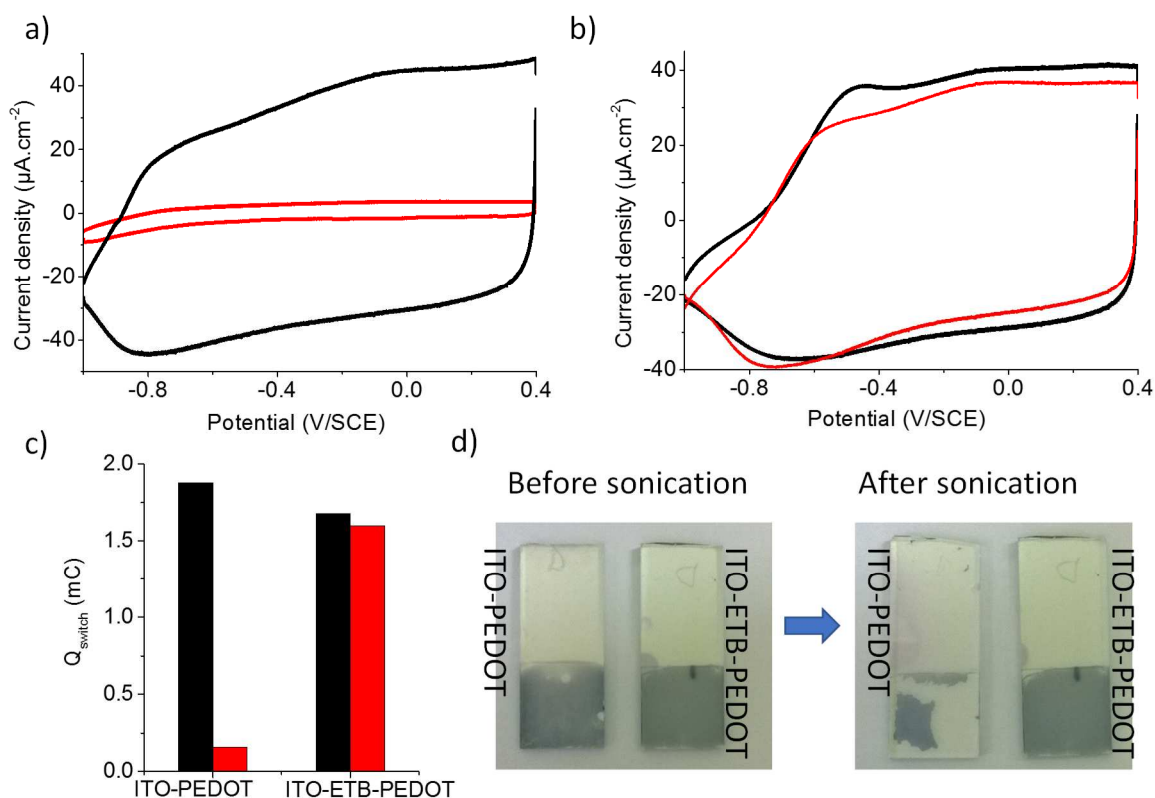
Figure 4. Cyclic voltammograms of PEDOT films obtained at constant current intensity ( 10^{-2} \text{mA}/\text{cm}^2 ) a) on bare ITO electrode before (black line) and after ultrasonication (red line), b) on ETB-modified electrode before (black line) and after ultrasonication (red line). c) Faradic and capacitive charges involved in the doping of the PEDOT film before (black) and after ultrasonication (red) for PEDOT on ITO and PEDOT on ETB-ITO electrodes. d) Optical images of PEDOT films on ITO (left) and ETB-ITO (right) before and after ultrasonication.
