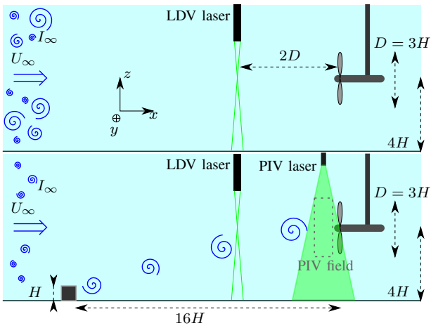
Fig. 2: Schematic representation of the two experimental setups: case A with I = 14\% (top) and the case B with I = 1.5\% and the presence of a wall-mounted cylinder (bottom). LDV measurements for case A, LDV and PIV measurements for case B.
