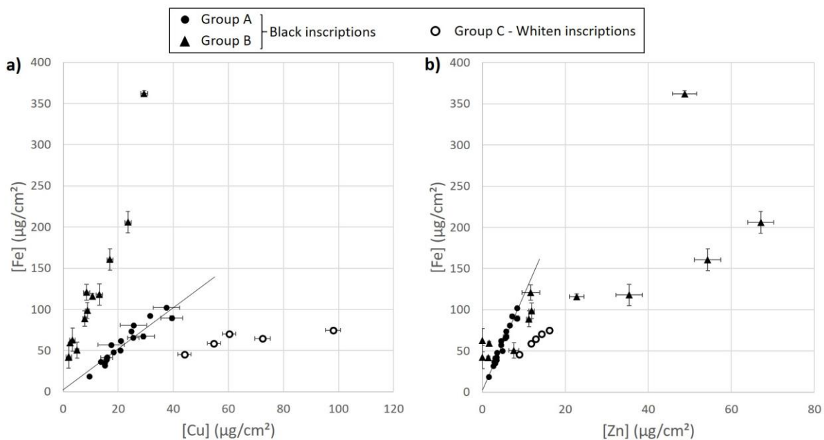
FIGURE 5. Iron concentration as a function of (a) copper and (b) zinc concentrations in the inks of all inscriptions of the corpus. Black dots correspond to black inscriptions and white dots to inscriptions showing a white layer on their surface.
