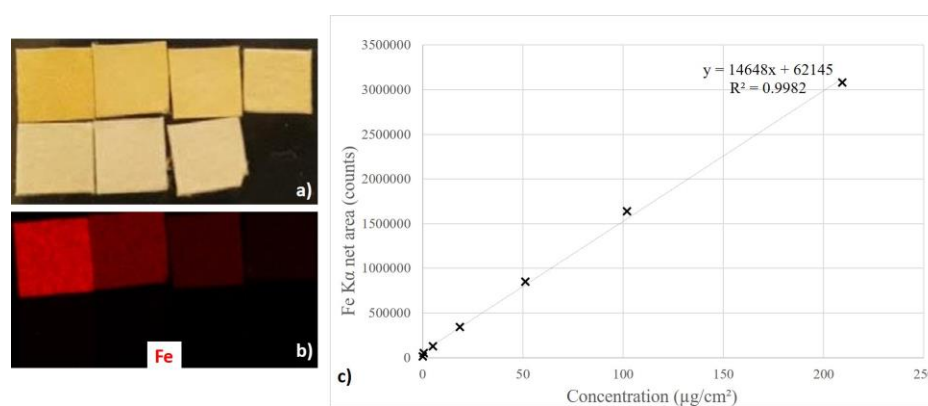
FIGURE 4. a) Visible picture of model samples made of paper test chart soaked in a solution of \text{FeSO}_4 at (from top left to bottom right) 100, 50, 25, 10, 2.5, 0.25 and 0.025 \text{g. L}^{-1} ; b) XRF map of the samples in (a) showing in red the distribution of the \text{K}\alpha line of iron; c) Calibration curve made from the net area of the peak of the \text{K}\alpha line of iron in the XRF spectrum as a function of the concentration of this element in the corresponding model sample.
