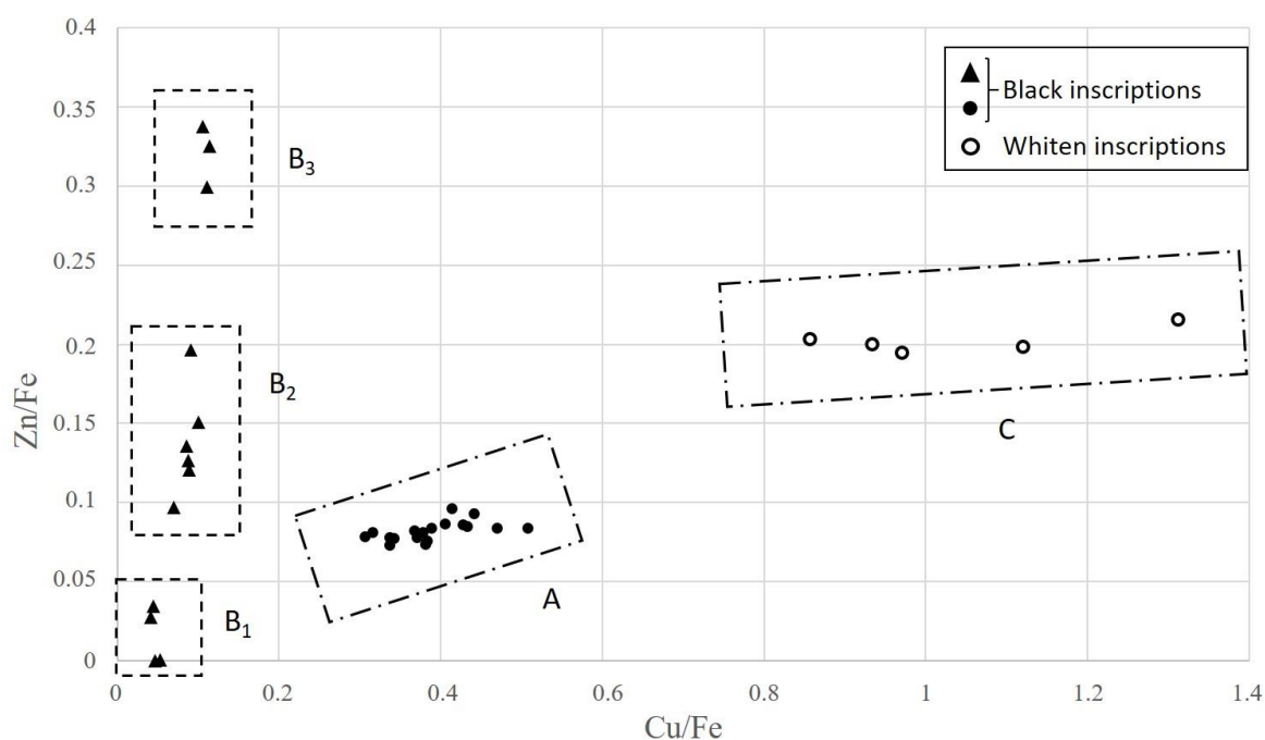
FIGURE 7. Mass ratio Zn/Fe as a function of Cu/Fe in the ink of all the inscriptions visible on the artefacts of the corpus. Black dots and triangles correspond to black inscriptions and white dots to inscriptions showing a white layer on their surface.
