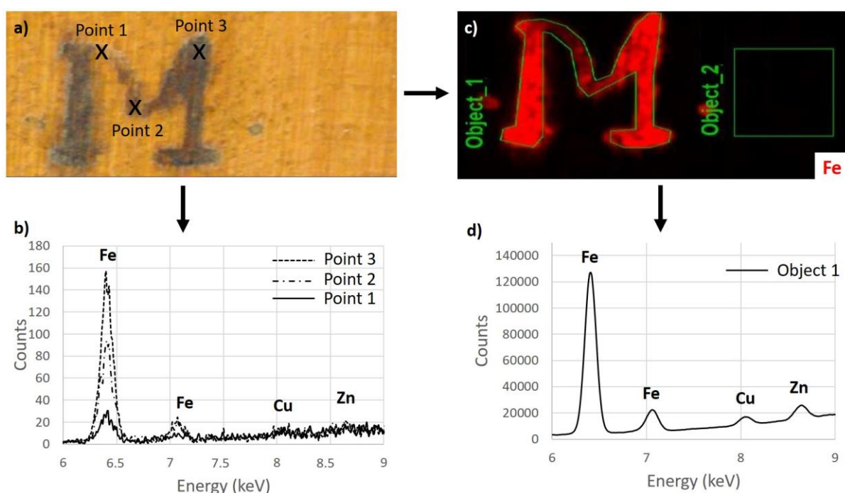
FIGURE 3. a) Visible picture of a detail of an inscription on the artefact E.903.18 showing the localization of the three single-point XRF analyses; b) XRF spectra extracted from the three positions in (a) centred on the K lines of iron, copper and zinc; c) XRF cartography of the K\alpha line of iron showing the 1400 pixels area on the ink (Object_1) and the corresponding one on the wood (Object_2); d) Sum spectrum extracted from the Object_1 in (c). XRF, X-ray fluorescence
