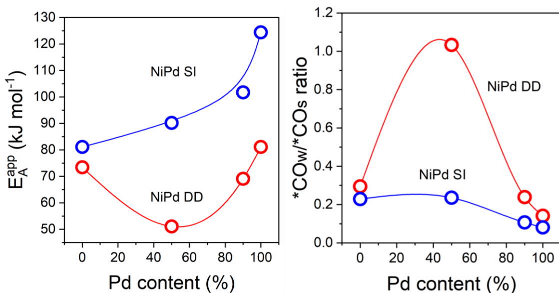
Figure 5: Correlation between the Apparent Activation Energies ( E_a^{app} ) and weakly to strongly adsorbed CO ratio ( *CO_w/*CO_s ) with Pd content.
