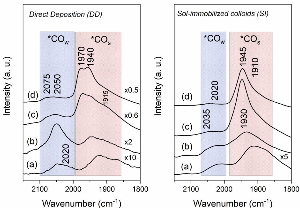
Figure 4: DRIFTS spectra of adsorbed CO at room temperature onto the reduced catalysts at 400°C, for 1h. (left) Ni x Pd y DD samples; (right) Ni x Pd y SI samples. (a) Ni 1 , (b) Ni 5 Pd 5 , (c) Ni 1 Pd 9 , (d) Pd 1 .
