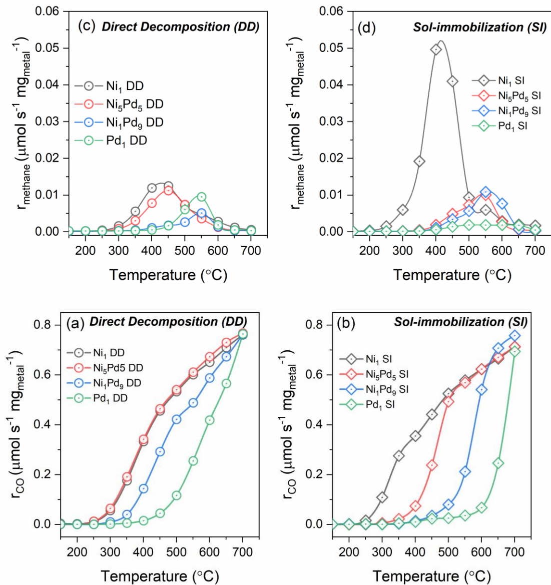
Figure 3: Rates of CO (a,b) and CH 4 (c,d) formation from RWGS as function of temperature for the series of NiPd catalysts prepared from Direct Decomposition, DD , (a,c) and Sol Immobilization, SI , (b,d) methodologies. Samples were pre-treated under H 2 at 400°C for 30 min; W_{\text{metal}}=0.5 mg of total metal (Ni+Pd); 1 CO 2 :4 H 2 :45 Ar.
