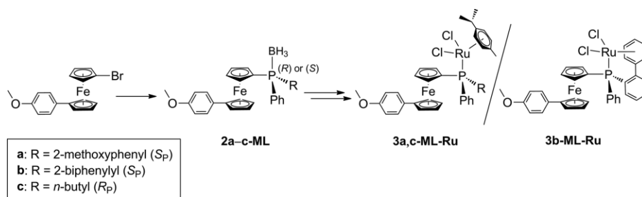
Scheme 1. Monomeric P -stereogenic ferrocenyl phosphine boranes 2a–c-ML and their corresponding monomeric ruthenium complexes 3a–c-ML-Ru . 3b-ML-Ru forms a tethered complex with loss of the p -cymene ligand when activated by light. [67,68]
