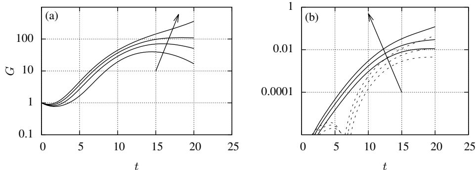
FIGURE 2. (a) Gain G as a function of the final time t for \epsilon \rightarrow 0 , \epsilon = 0.015, 0.0153, 0.016 , for \alpha_{opt} = 0.93 , \beta_{opt} = 1.44 (obtained by choosing T = 20 as target time for the optimization) and Re = 400 . (b) Energy of the mean flow modification, E_U (—) and E_W (---), for \epsilon = 0.015, 0.0153, 0.016 . The arrows display increasing values of \epsilon .
