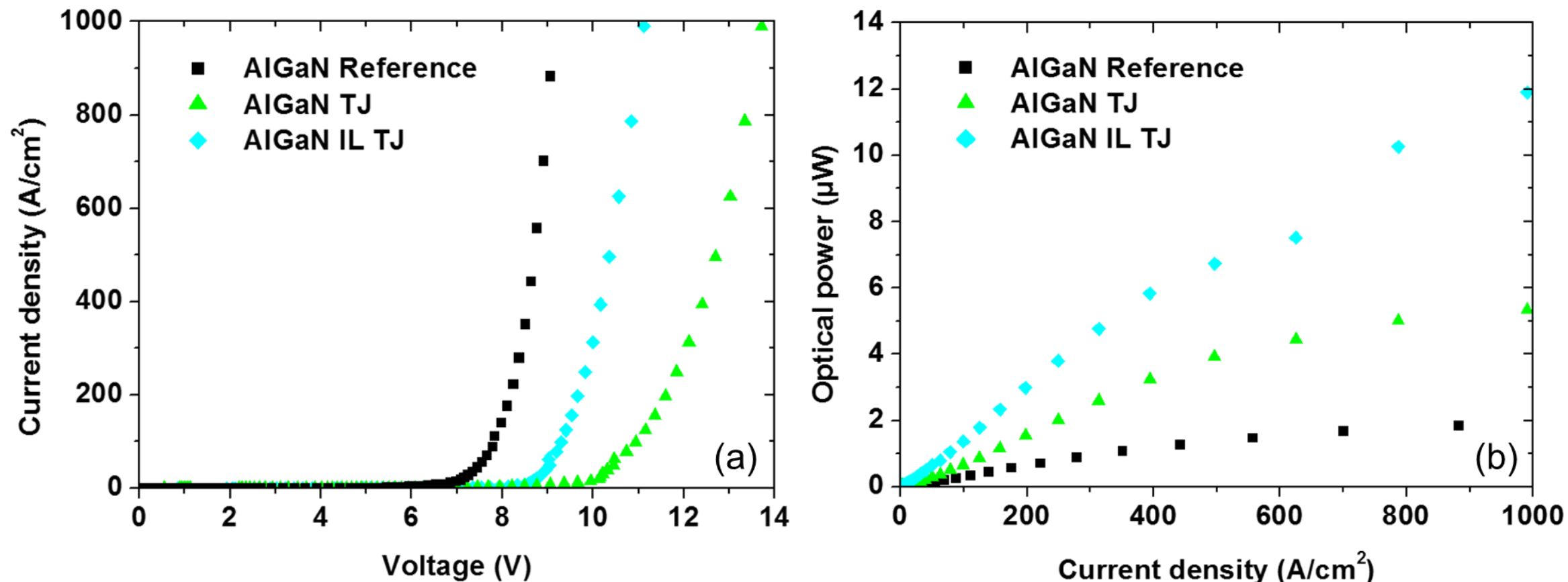
Figure 6. Current density versus bias (a) and optical power (b) for the AlGaN TJs and their AlGaN reference without TJ. The LEDs had an area of 0.0016 \text{ mm}^2 .
