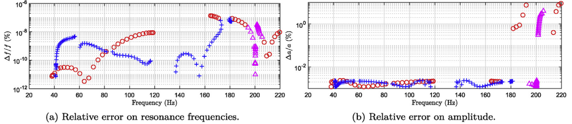
Fig. 10. Evaluation of the error for the reduction of the heterogeneous beam model.
