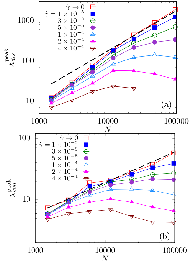
FIG. 4: The peak values of the disconnected (a) and connected (b) susceptibilities, \chi_{\text{dis}}^{\text{peak}} and \chi_{\text{con}}^{\text{peak}} , as a function of the system size N for 3D stable glasses with T_{\text{ini}} = 0.062 . The dashed lines correspond to the scaling behaviors observed in the AQS limit, \chi_{\text{dis}}^{\text{peak}} \propto N and \chi_{\text{con}}^{\text{peak}} \propto N^{1/2} . Departure from the AQS limit arises at smaller N when \dot{\gamma} increases, indirectly revealing a crossover lengthscale \xi controlled by the shear rate \dot{\gamma} .
