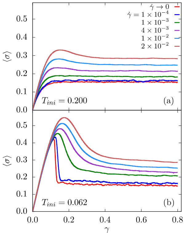
FIG. 2: Average stress strain curves for 3D glasses for N = 12000 (a) at high initial preparation temperature T_{ini} = 0.200 , and (b) at low initial preparation temperature T_{ini} = 0.062 . The data denoted \dot{\gamma} \rightarrow 0 are measured using AQS simulations.
