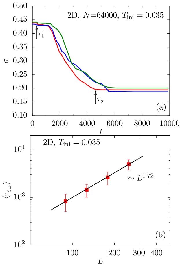
FIG. 8: (a) Stress relaxation during the largest stress drop for stable glasses using physical steepest descent dynamics. The times \tau_1 and \tau_2 describe the beginning and the end of the shear band formation for the red curve. (b) The averaged duration of the shear band formation, \langle \tau_{SB} \rangle = \langle \tau_2 - \tau_1 \rangle increases algebraically with the system size with an exponent \beta \approx 1.72 that is then used in Fig. 7.
