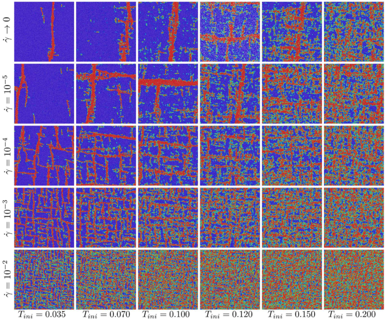
FIG. 6: Snapshots of the non-affine D_{\min}^2 field immediately after yielding (at the strain \gamma_A ) for several T_{\text{ini}} and various shear rates \dot{\gamma} for the 2D system with N = 64000 ( L = 253 ). An increasing number of shear bands is formed as the strain rate increases, which form a checkerboard pattern for low T_{\text{ini}} with characteristic lengthscale \langle \xi \rangle .
