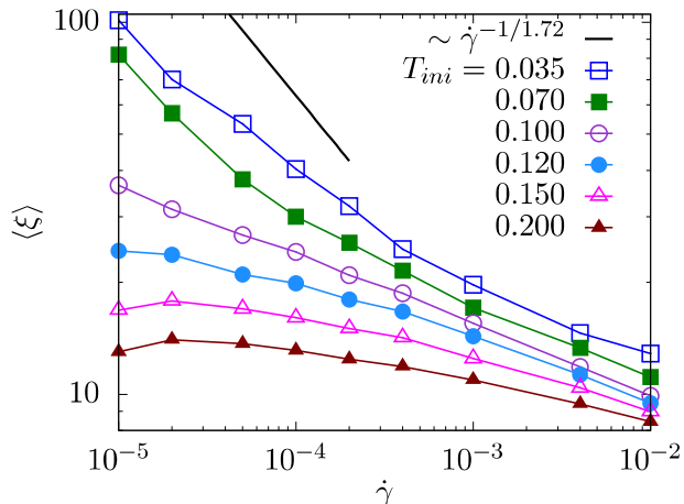
FIG. 7: Evolution of the typical distance between shear bands with the shear rate for the 2D model at various value of T_{ini} . The solid straight line corresponds to the scaling predicted by Eq. (7) using the exponent \beta = 1.72 measured in Fig. 8, which should hold for low T_{ini} and small \dot{\gamma} .
