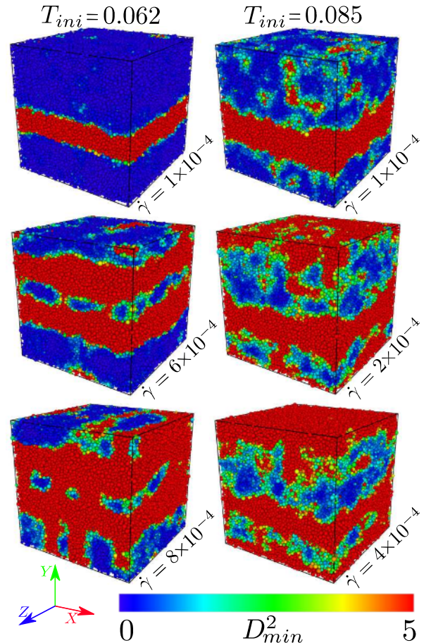
FIG. 5: Snapshots of the non-affine D_{\min}^2 field immediately after yielding (at the strain \gamma_A shown in Fig. 3) for two different T_{\text{ini}} and various shear rates \dot{\gamma} for the 3D system with N = 96000 . An increasing number of shear bands is observed as the strain rate increases.
