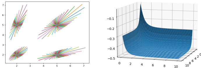
FIGURE 2. On the left, geodesic balls and and on the right, sectional curvature of the manifold of beta distributions ( n=2 ).
