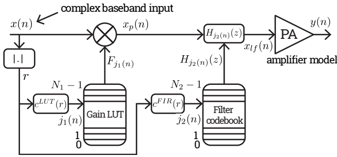
Fig. 1: Complex gain FLUT predistortion followed by PA.
