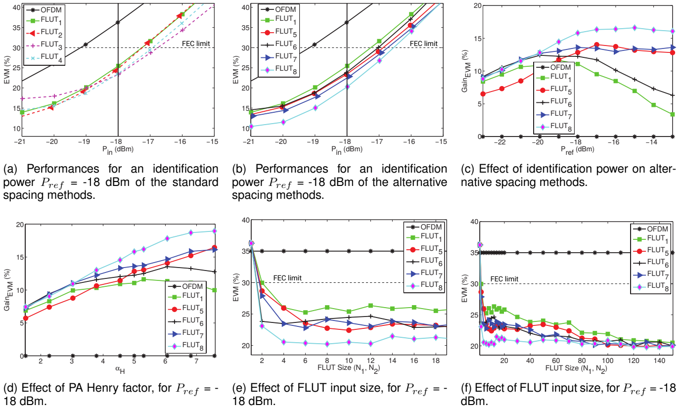
Fig. 3: Standard and alternative spacing methods.
