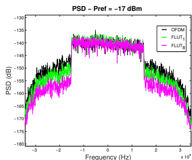
Fig. 5: Power Spectral Density of the received signal (original system and linearized systems FLUT_1 , FLUT_8 ).
