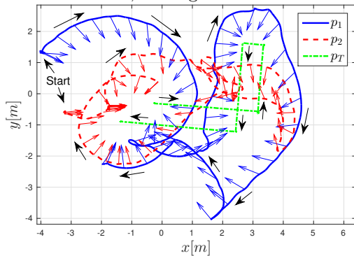
Figure 9. Two quadrotors tracking a moving UGV, colored arrows represent the front axes of each UAV.
