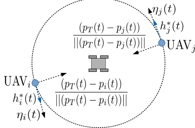
Figure 4. Circular path generation using perpendicular vectors on the optimization cost function.
