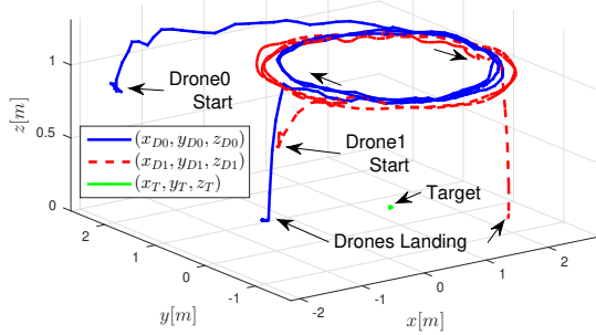
Figure 7. Two quadrotors surrounding a static UGV by describing circles.
