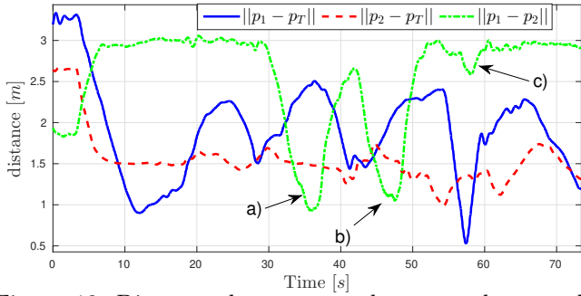
Figure 13. Distances between quadrotors and to the UGV target are recovered disturbances.
