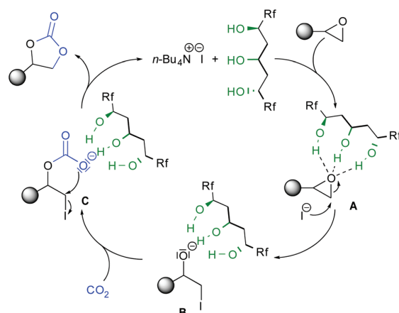
Scheme 3 Proposed mechanism for the epoxide opening.
