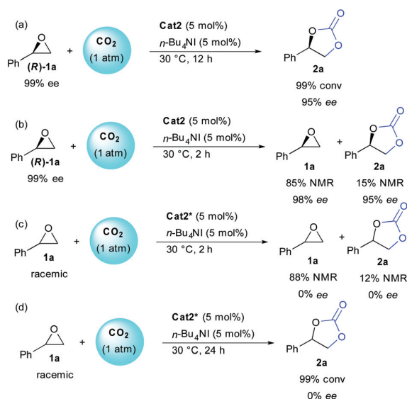
Scheme 2 Stereochemical outcome of the epoxide opening.
