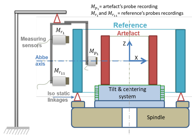
Figure 1. Partial schematic of the DMT architecture of the LNE machine
