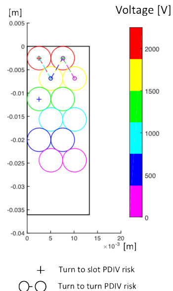
Figure 19. Initial winding configuration in the motorette; turn to turn & turn to slot PD risk
