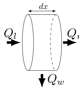
Figure 4. Mass balance in a slice of an idealized airway (cylinder). The variation of oxygen concentration in the slice depends on the balance between the oxygen flow entering the slice and getting out of the slice.
