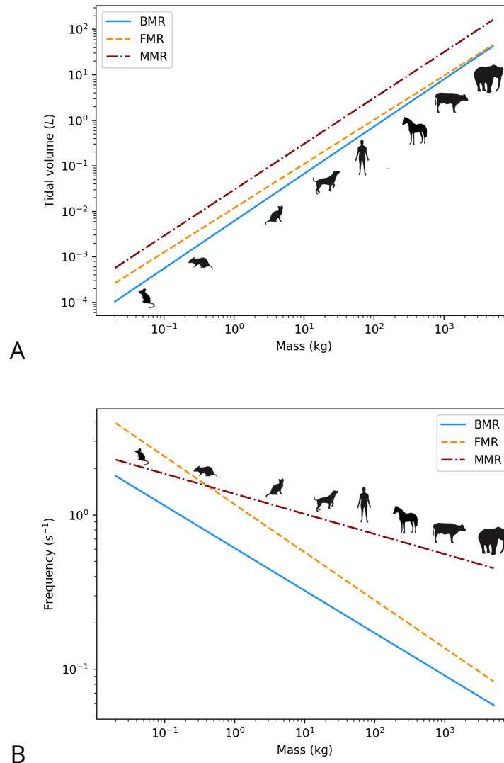
Figure 2. A: Predicted tidal volume as a function of the mammal mass (log-log). Solid line: BMR, V_T^{\text{BMR}} \simeq 6.1 M^{1.04} ml; dashed line: FMR, V_T^{\text{FMR}} \simeq 11.8 M^{0.97} ml, dash-dotted line: MMR, V_T^{\text{MMR}} \simeq 29.7 M^{1.01} ml. B: Predicted breathing frequency as a function of the mammal mass (log-log). Solid line: BMR, f_b^{\text{BMR}} \simeq 0.61 M^{-0.27} Hz; dashed line: FMR, f_b^{\text{FMR}} \simeq 1.17 M^{-0.31} Hz, dash-dotted line: MMR, f_b^{\text{MMR}} \simeq 1.37 M^{-0.17} Hz. A larger dead volume at exercise (Haverkamp et al., 2005) makes the oxygen source for diffusion slower to deplete. This might lead to a decrease in the optimal breathing rate, depending on the increase of the oxygen need. As a consequence, for small mammals, our model predicts breathing frequencies at MMR smaller than breathing frequencies at FMR.
