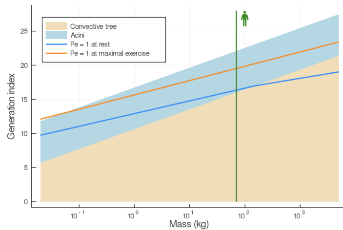
Figure 3. Localization of the transition between convective and diffusive transport of oxygen in the lung as a function of animal mass (logarithmic scale). The lines correspond to the localizations of that transition at BMR (rest, blue line) and MMR ( \dot{V}_{O_2}^{\max} , orange line). The vertical green line corresponds to human mass (70 kg). The lower beige region corresponds to the convective zone of the lung and the upper blue region corresponds to the exchange surface (acini). Small mammals tend to transport oxygen mainly by convection. Hence, there is no screening effect (Sapoval et al., 2002) affecting their exchange surface. Their oxygen pressure gradients between alveoli and blood are maximal everywhere, making their pulmonary system very efficient. To the contrary, due to the screening effect, large mammals use only a small portion of their exchange surface at rest. Hence, large mammals have a large reserve of exchange surface available for higher metabolic rates. Increasing the ventilation amplitude decreases the screening effect. Hence, the pulmonary system of large mammals is more efficient at exercise than at rest.
