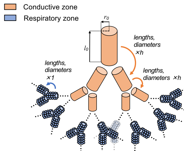
Figure 1. Illustration of the lung model used in this work. Our model is based on the assembly of self-similar trees with symmetric bifurcations that mimic the two functional zones. The tree in beige mimics the bronchial tree, where oxygen is only transported along the branches. The tree in blue mimics the acini, where oxygen is transported along the branches and also captured in the alveoli that cover the walls of the branches. The model of oxygen transport depends only on airways lengths and diameters but not on airways spatial distribution in the lungs. Hence, branching angles and branching planes orientations are not accounted for in this work.
