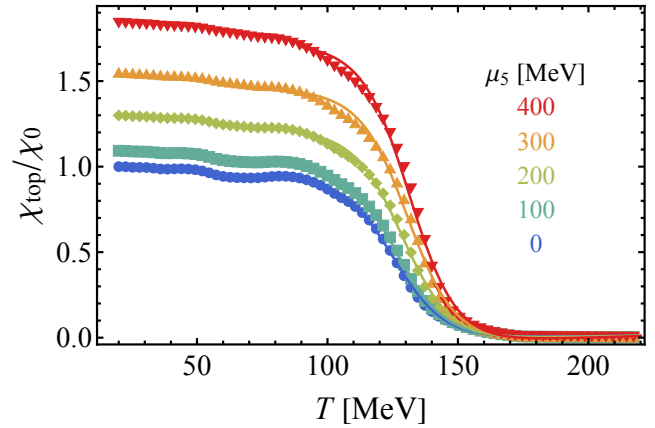
Figure 4: Topological susceptibility (56) versus temperature, in units of the vacuum susceptibility \chi_0 (57). Conventions for colors and symbols are the same used in Fig. 1. The solid lines represent the best fits by the function (54).
